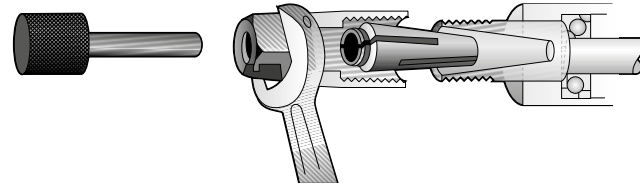
Figure 16. Collet chuck.
