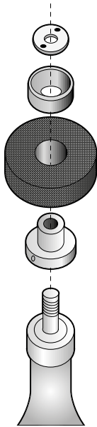
Figure 27. Flange assembly
