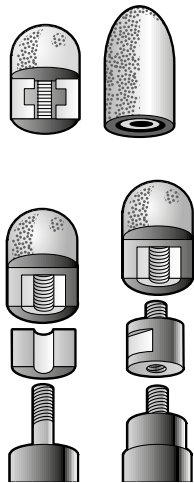
Figure 29b. Cone wheel
