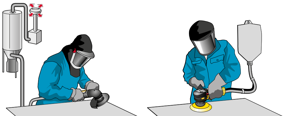
Figure 52. Spot suction
